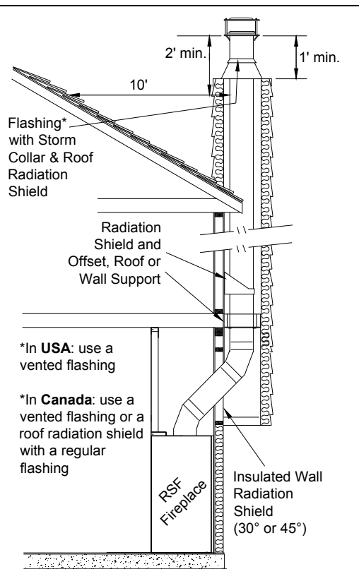
Figure 9 Offset Chimney Through a Wall Example
