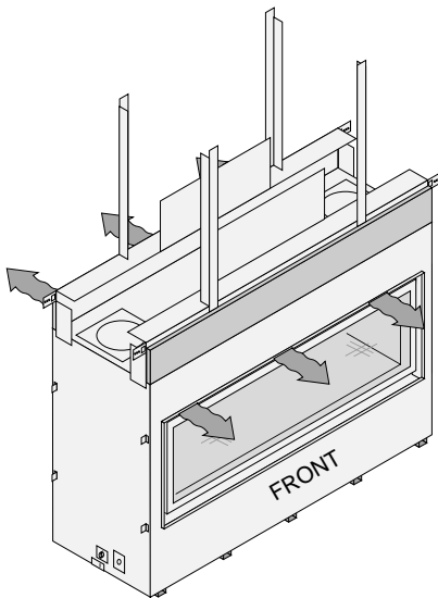
Divided Air Flow (stock)
