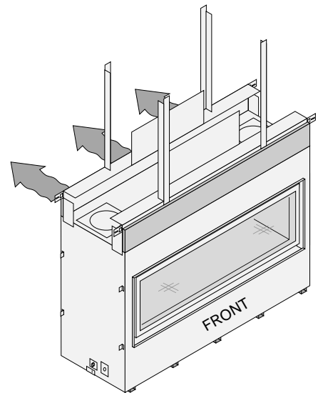
Air Flow to Back
